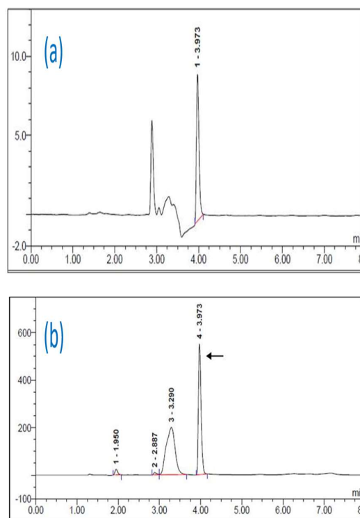
Figure 4. HPLC for structure determination of the extracted intermediate. (a) HPLC chromatogram of the extracted intermediate. (b) HPLC chromatogram of 500ppb ETU showing a peak at 3.973 minutes. (b)
