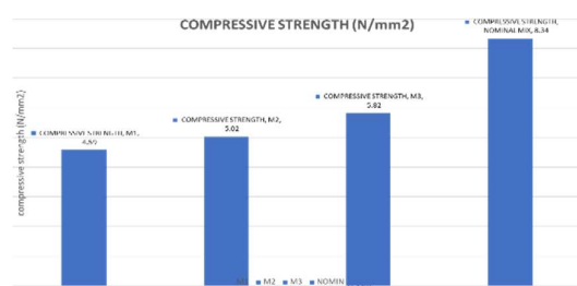
Figure 4. Compressive strength test result graph
