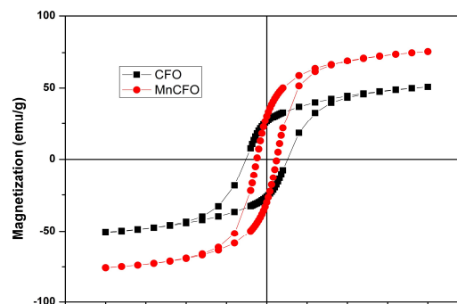
Fig 7. M-H loop of cobalt ferrite & manganese doped (a) \text{CoFe}_2\text{O}_4 (b) \text{CoMn}_{0.125}\text{Fe}_{1.875}\text{O}_4 , sample cobalt ferrite nanoparticles.
