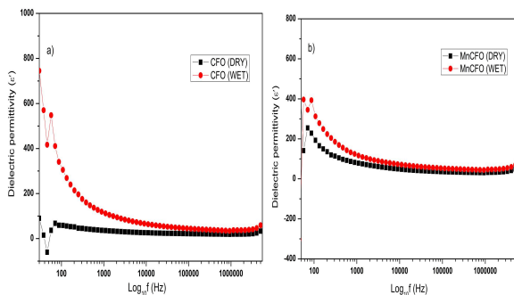
Fig 8. Dielectric constant with frequency for dry and wet hydroelectric cells of (a) \text{CoFe}_2\text{O}_4 (b) \text{CoMn}_{0.125}\text{Fe}_{1.875}\text{O}_4 . increased for wet HEC as compared to dry HEC at low frequency range. The \epsilon' values have become almost constant at high frequency range. This behaviour in the variation of \epsilon' values is mainly due to rise in ionic and space charge polarization due to dissociated water molecules [26].
