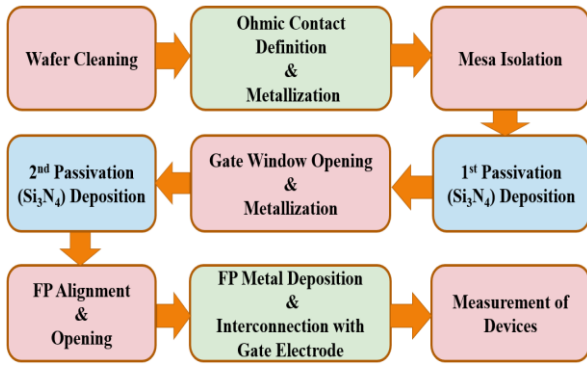
Figure 2. Flow chart of the fabrication of AlGaN/GaN HEMT devices.
