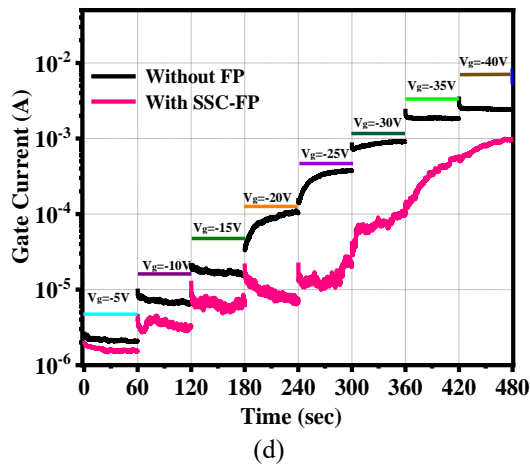
(d) Figure 5. Post reverse bias step stress scheme, (a) Output characteristics, (b) & (c) shows transfer characteristics, and (d) gate current as a function of transient time.
